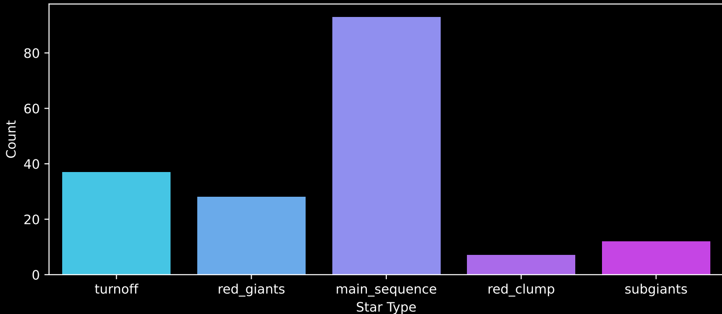
APOGEE DR17 Field: [178+42_MGA] Count plot of Star Type
