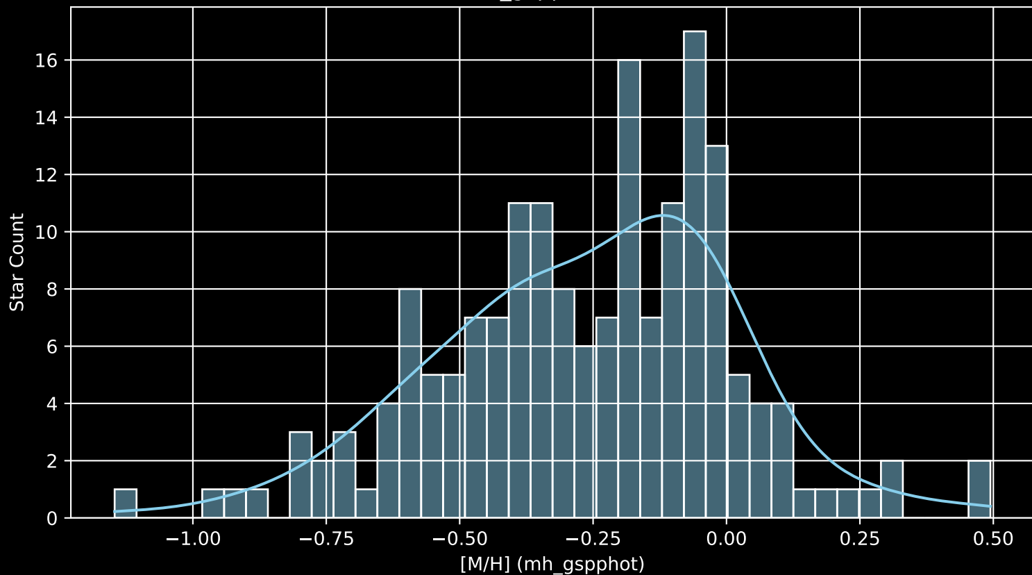
APOGEE DR17 Field: [178+42_MGA [M/H] (mh_gspphot) (n= 177)
