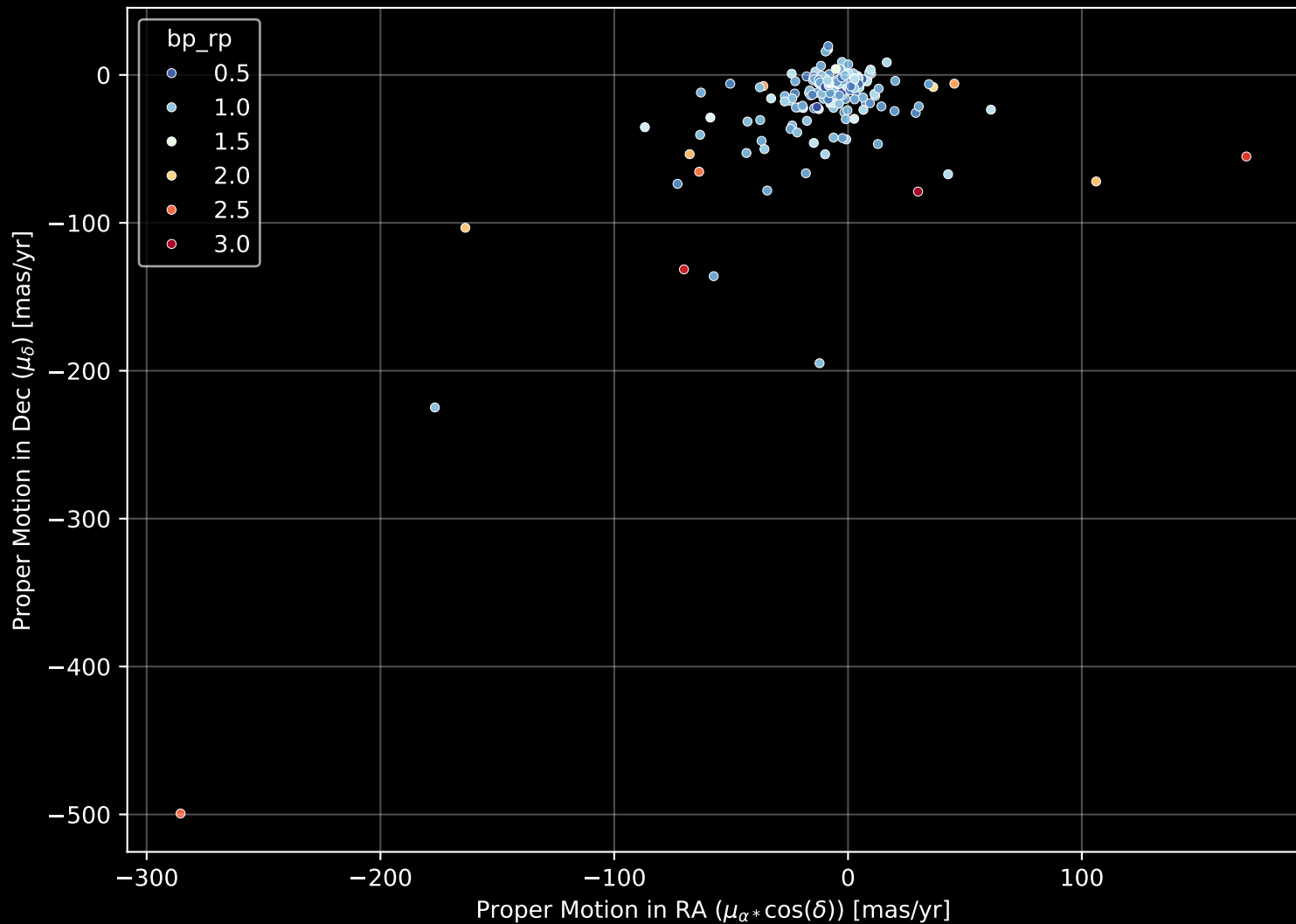
APOGEE DR17 Field: [178+42_MGA] Proper Motion Diagram (n= 177)
