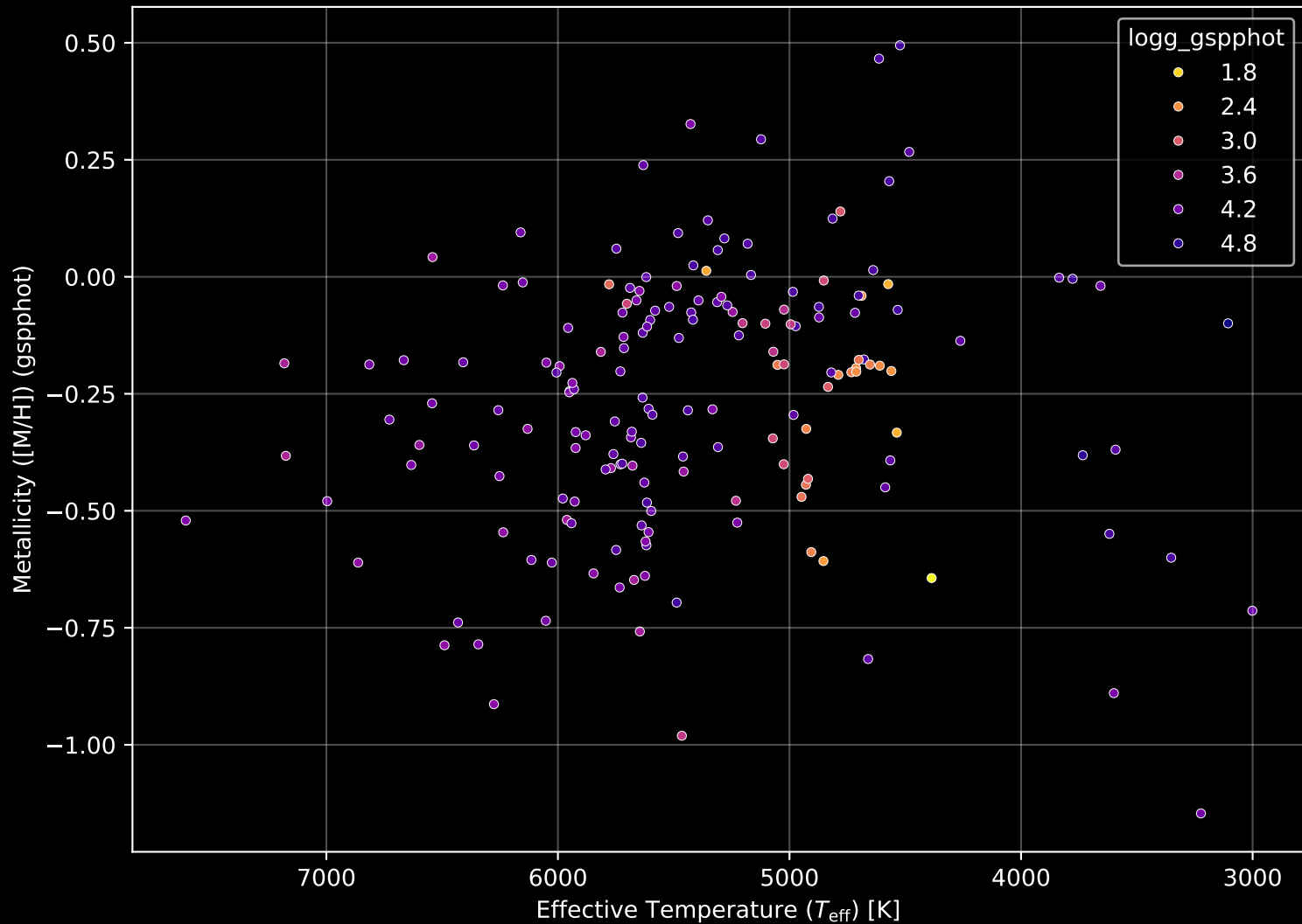
APOGEE DR17 Field: [178+42_MGA] Stellar Population Parameters (n= 177)
