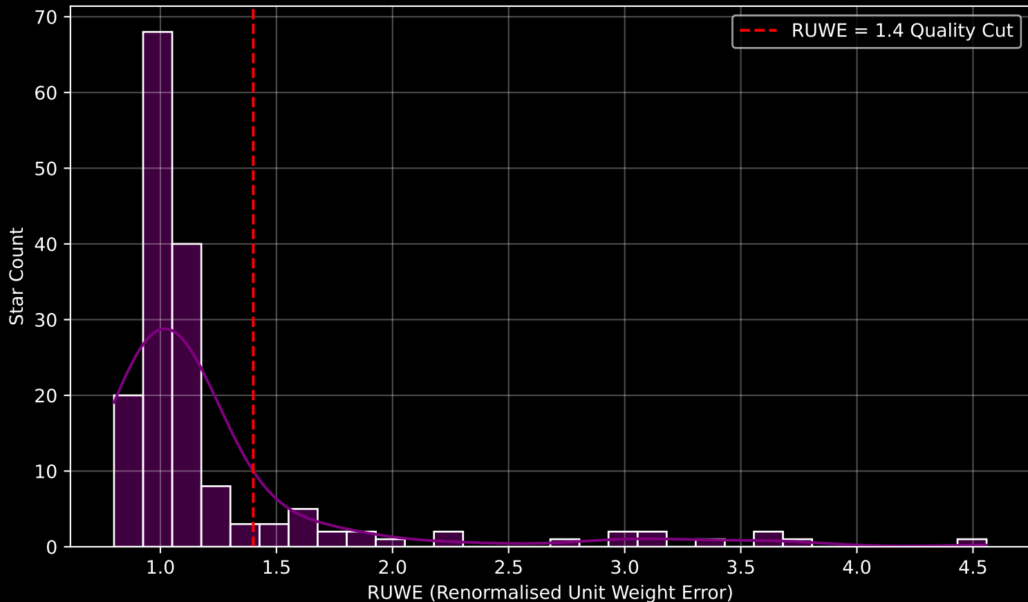
GAPOGEE DR17 Field [178+42_MGA] RUWE Distribution (n= 164)
