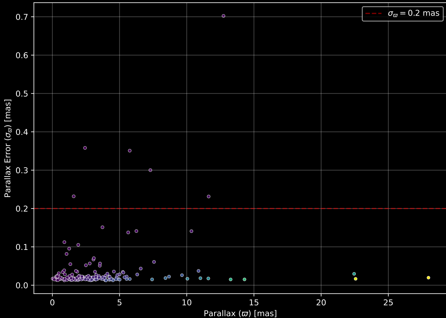
APOGEE DR17 Field: [178+42_MGA] Parallax Quality (n= 177)
